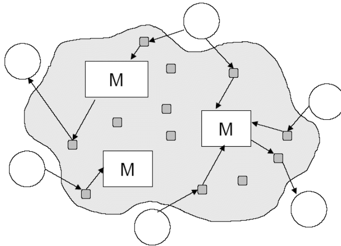
Figure 2.2: Topologia
