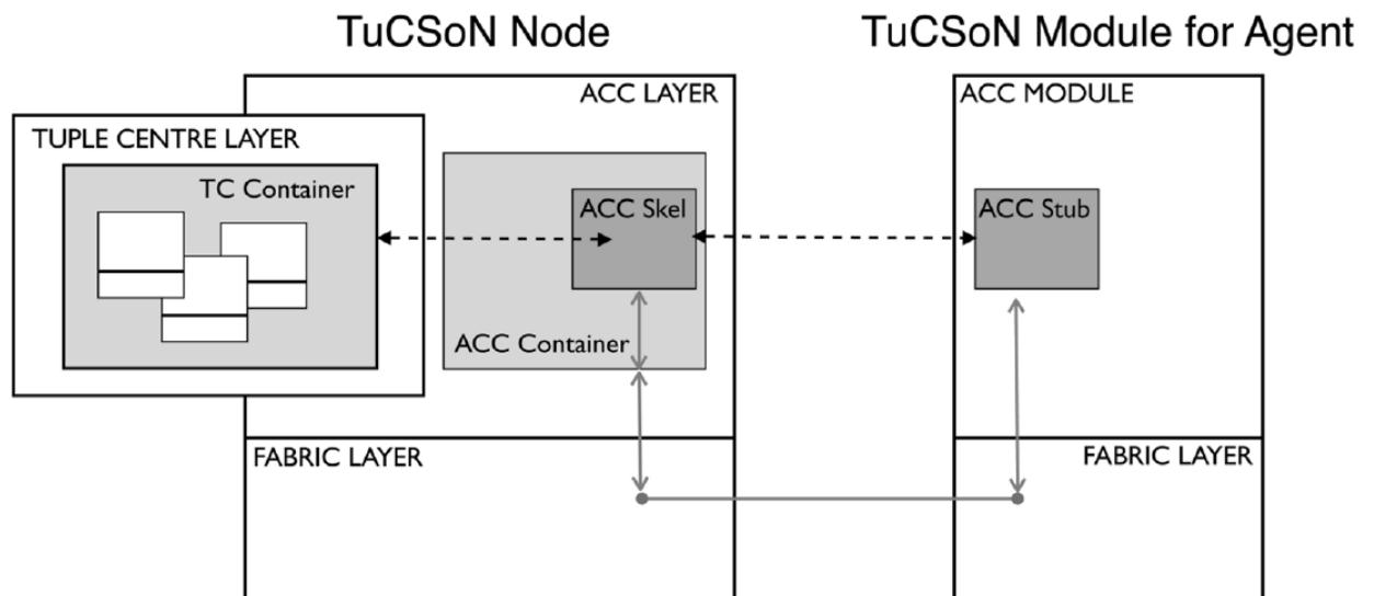
Figure 2.4: Topologia ACC
