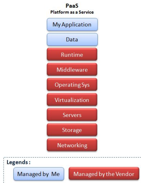
Figure 1.3: Platform-as-a-Service (PaaS)
