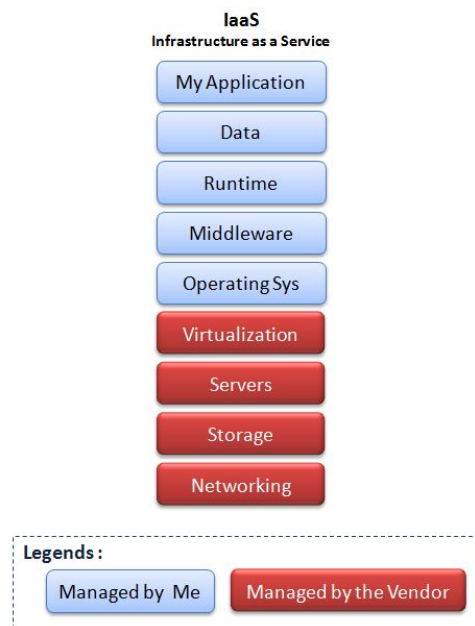
Figure 1.2: Infrastructure-as-a-Service (IaaS)
