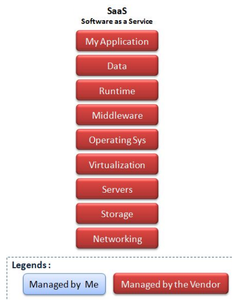
Figure 1.4: Software-as-a-Service (SaaS)
