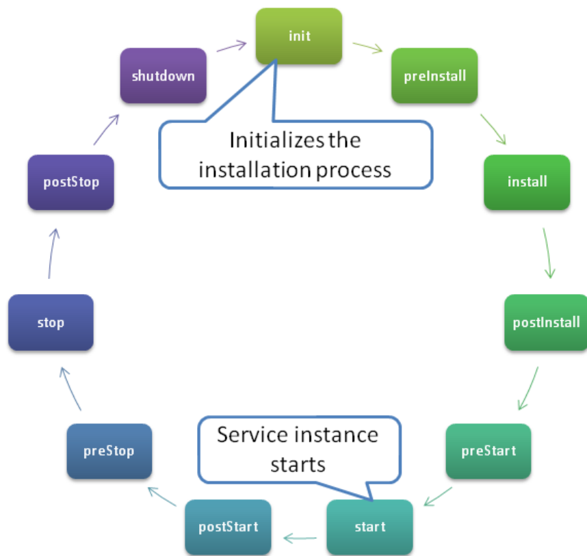
Figure 4.4: service instance lifecycle
