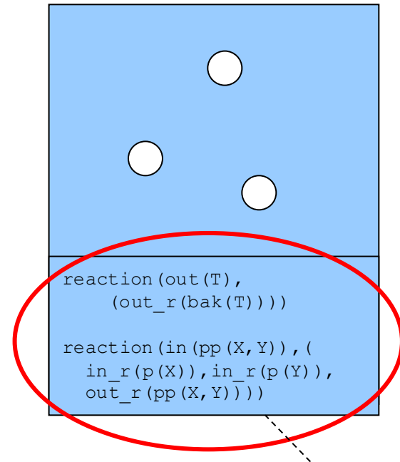
specification tuples (ReSpecT language)
