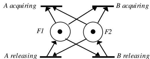
Figure 8. The core of the interaction protocol at the resource perception level
