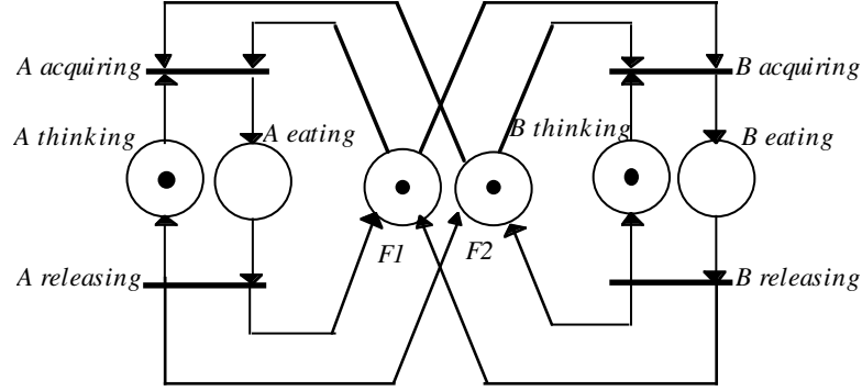
Figure 5. A simple two-philosopher system
