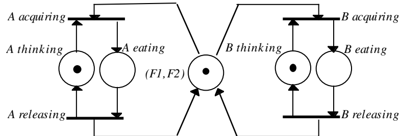
Figure 6. The two-philosopher system from a philosopher viewpoint
