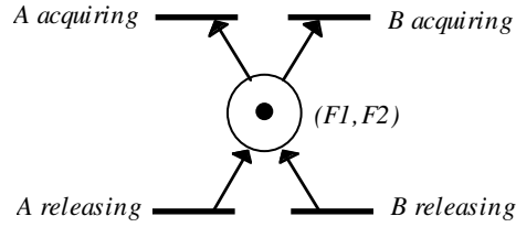
Figure 7. The core of the interaction protocol at the agent perception level
