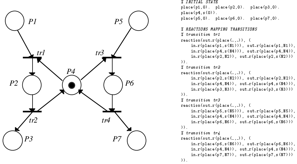
Figure 1. The initial state of a Petri Net represented as place/2 tuples, along with four reactions representing the four net's transitions
