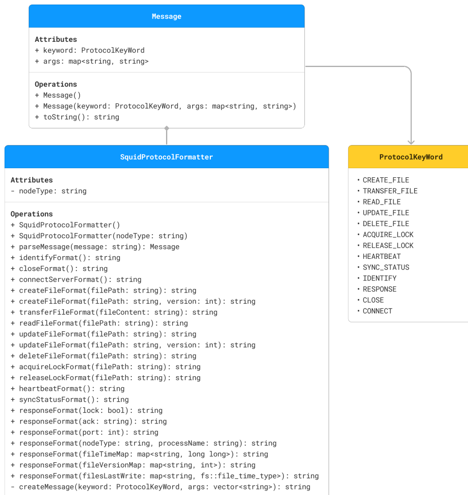
Figure 12: Formatter and Message classes
