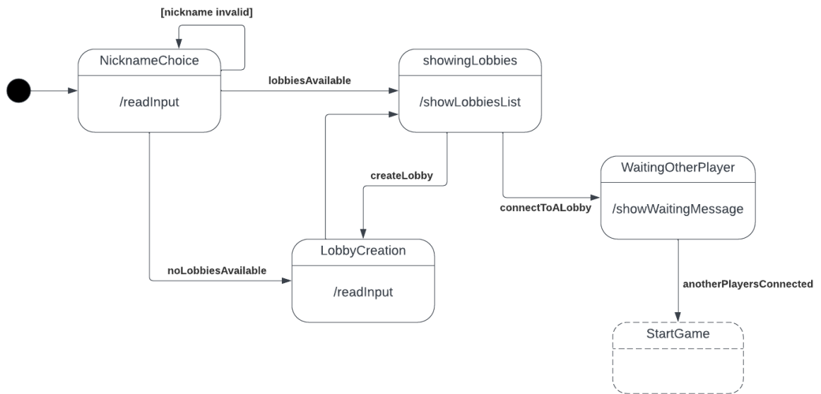
Figure 4: Lobby State Diagram
