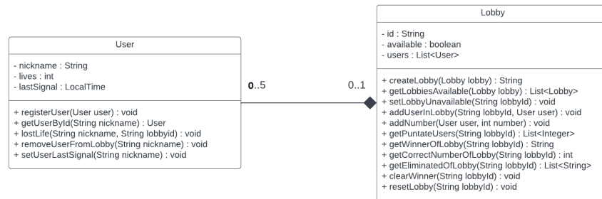
Figure 3: Class Diagram
