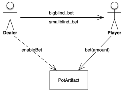
Fig. 8. Blind_Bet state
