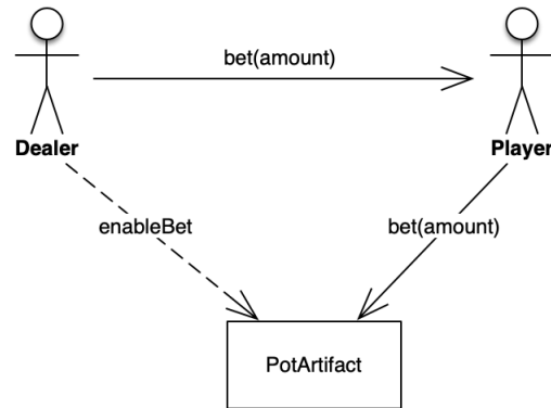
Fig. 10. Preflop_Bet state
