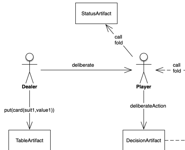
Fig. 11. Flop/Turn/River state
