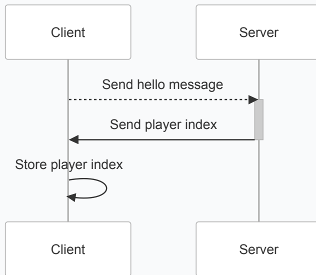
Figure 3.7: Sequence diagram of client-server handshake.
