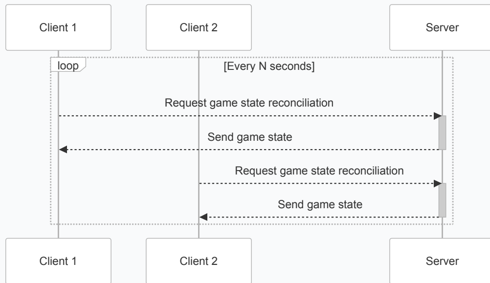
Figure 3.9: Sequence diagram of the game state reconciliation.
