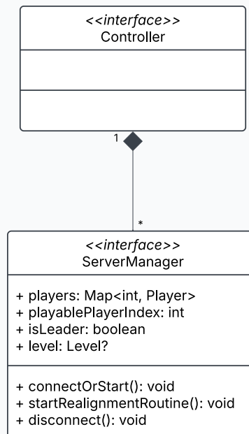
Figure 3.2: Position of ServerManager in the MVC architecture.
