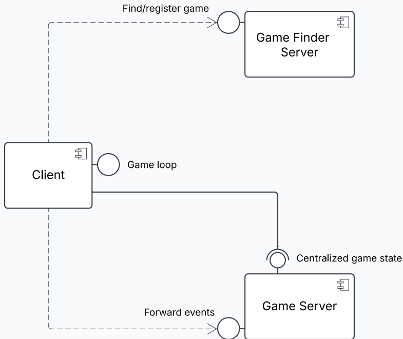
Figure 3.1: Component diagram of the infrastructure.
