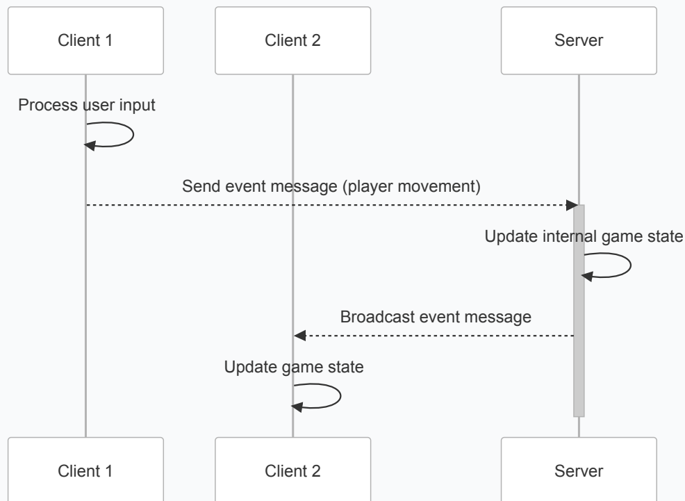
Figure 3.8: Sequence diagram of input events.
