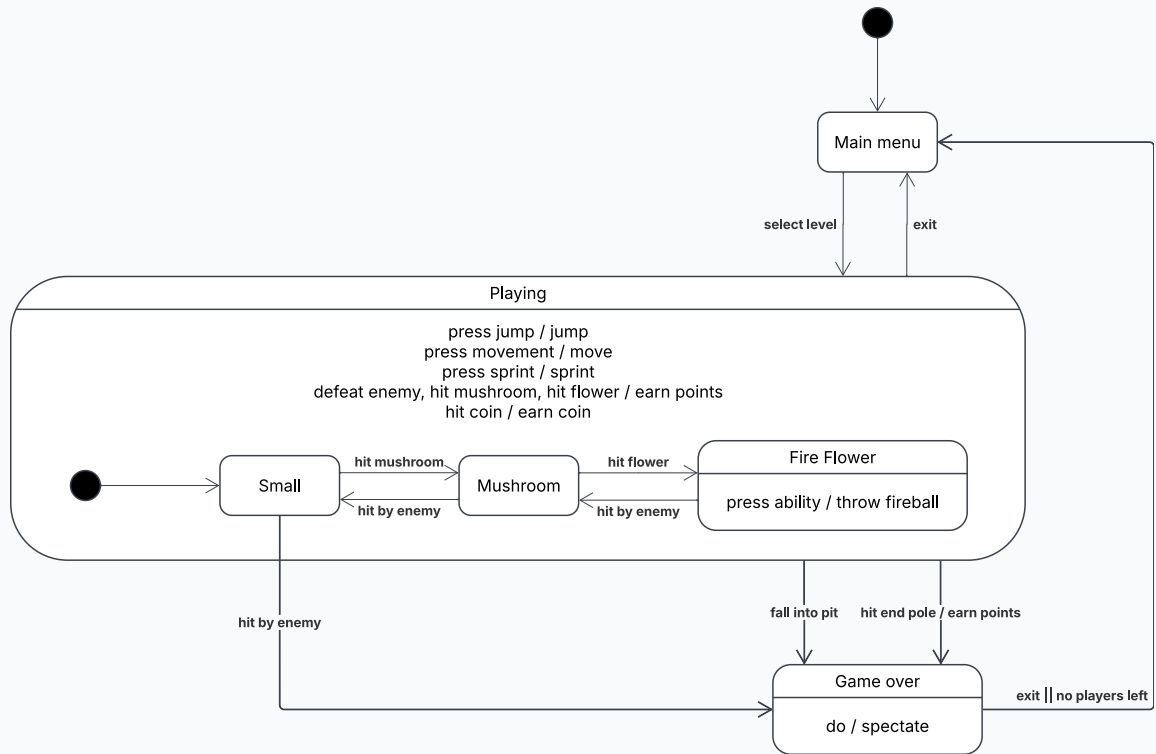
Figure 3.10: State diagram of the player lifecycle.
