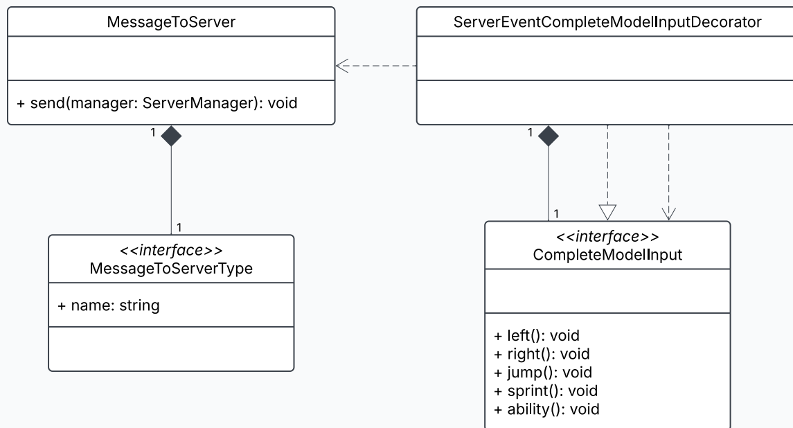
Figure 3.3: Class diagram of the input decorator.
