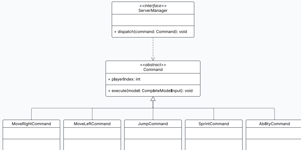
Figure 3.4: Class diagram of the command hierarchy.
