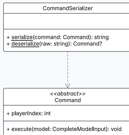
Figure 3.5: Class diagram of the command (de)serializer.
