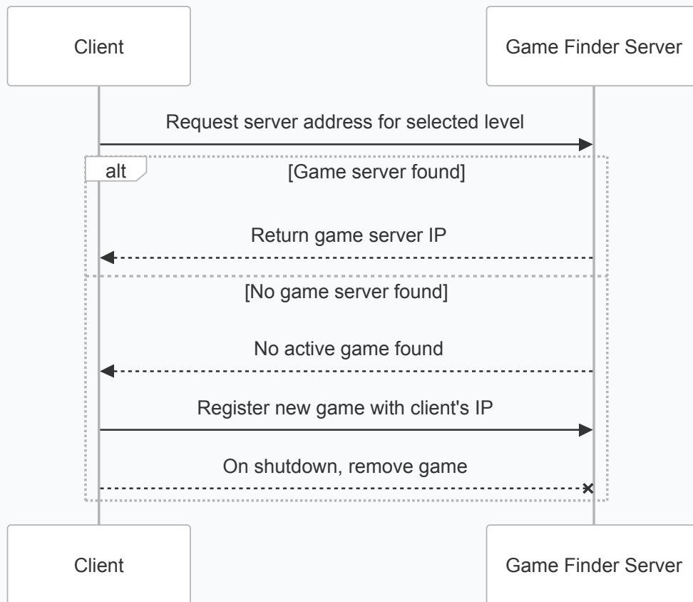
Figure 3.6: Sequence diagram of game finding.
