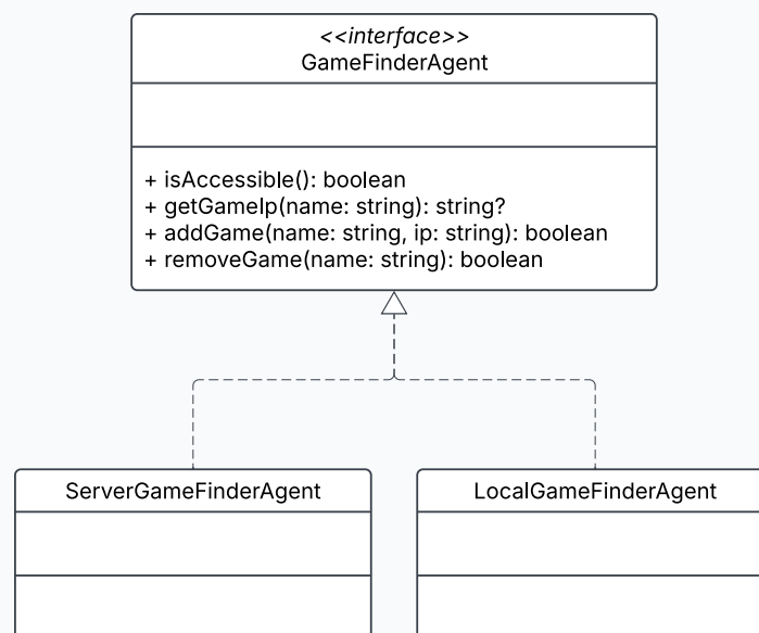
Figure 4.1: Class diagram of the game finder agent hierarchy.
