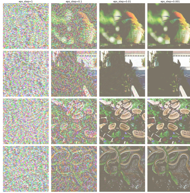
Figure 3: Grid search visualization results for PGD.
