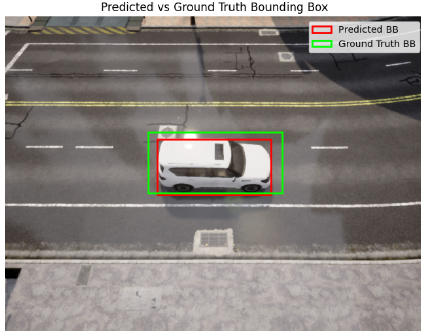
Figure 15: Original dataset car detection (red) and ground truth (green).
