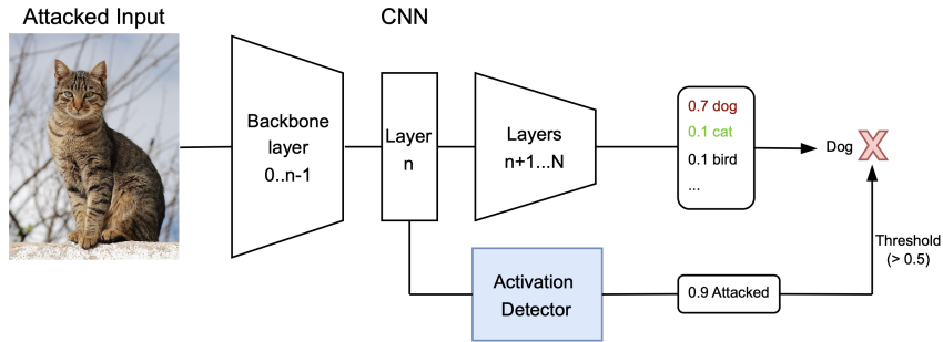
Figure 2: Activation detector schema drawn by us for the sake of clarity.
