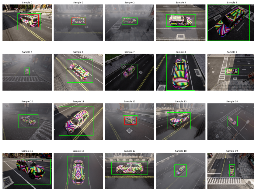
Figure 16: Adversarial dataset car detection (red) and ground truth (green) on different samples.
