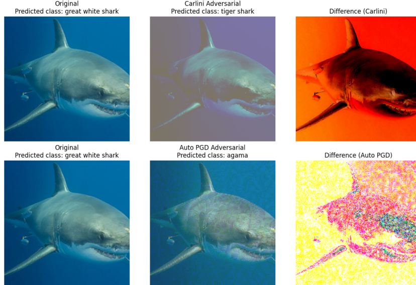
Figure 1: Neural network fooling with Carlini and PGD attacks.
