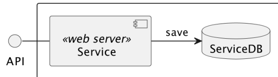
Figure 3: Microservice components
