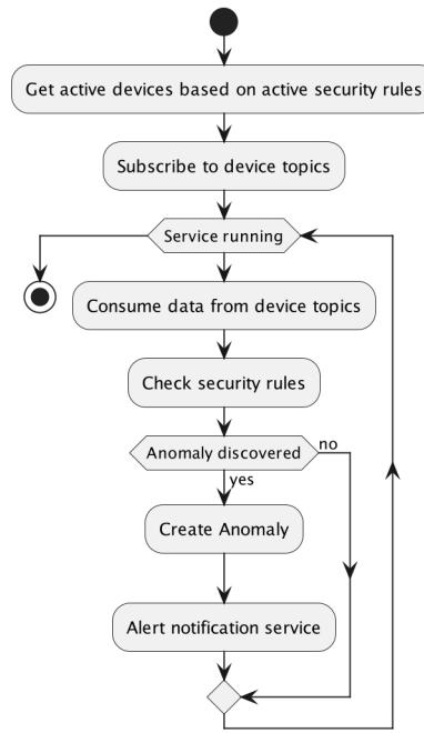
Figure 7: Alarm service activity diagram
