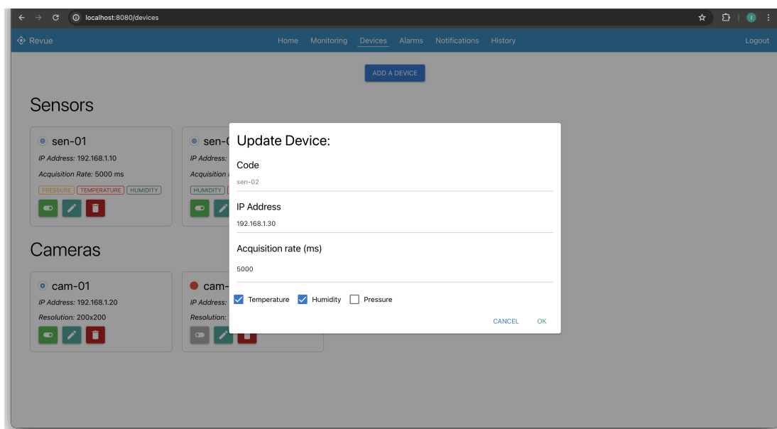
Figure 16: Updating a device
