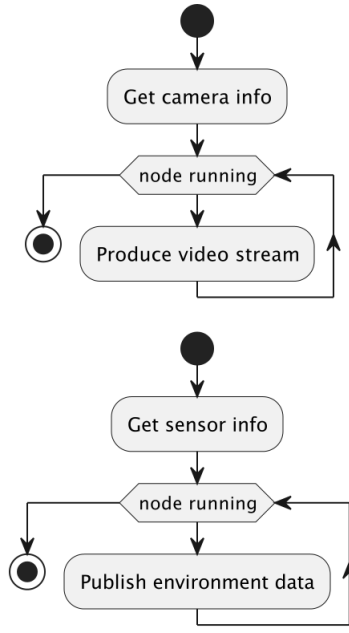
Figure 8: Device activity diagram
