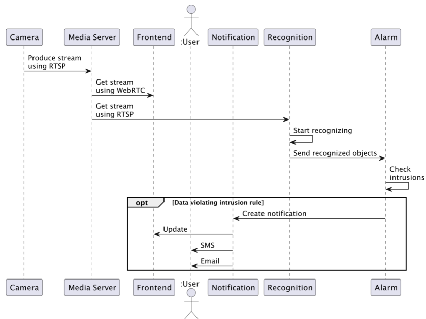
Figure 10: Video stream sequence diagram
