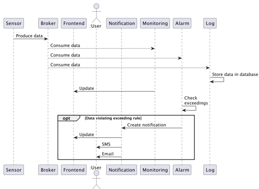
Figure 11: Sensor data sequence diagram
