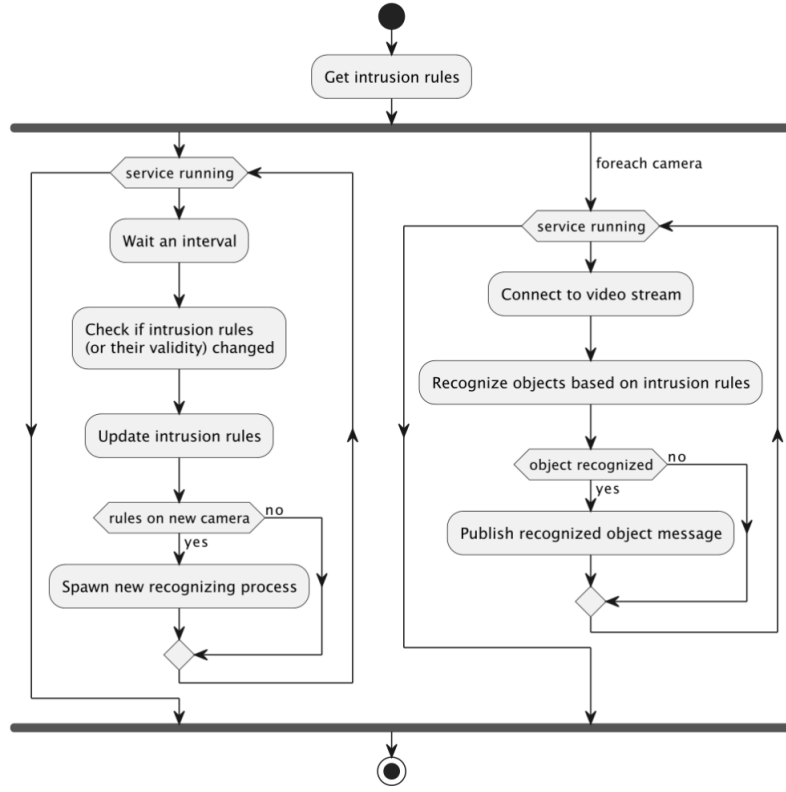
Figure 6: Recognition service activity diagram
