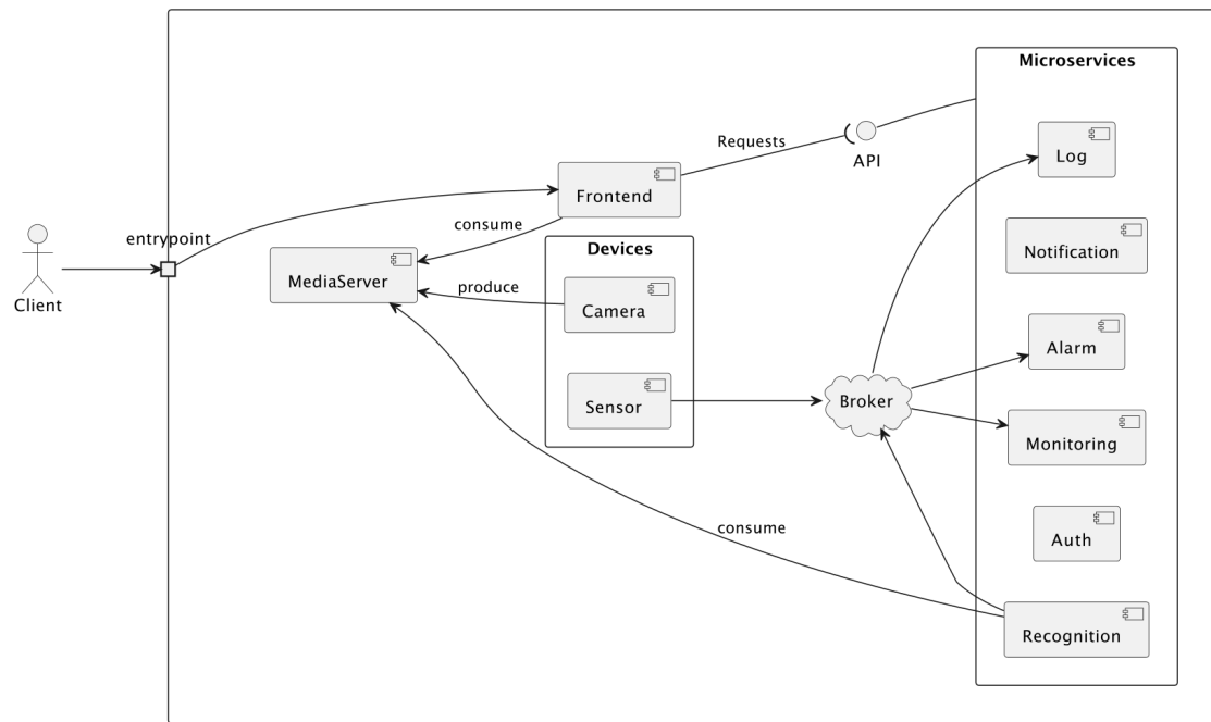
Figure 4: Revue Architecture
