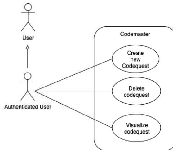
Figure 3: Codequest management use case diagram
