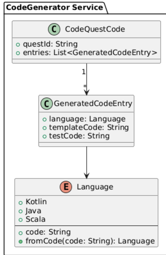
Figure 14: Code generator class diagram
