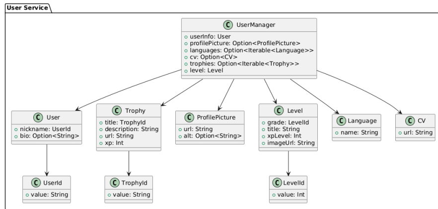
Figure 9: User class diagram
