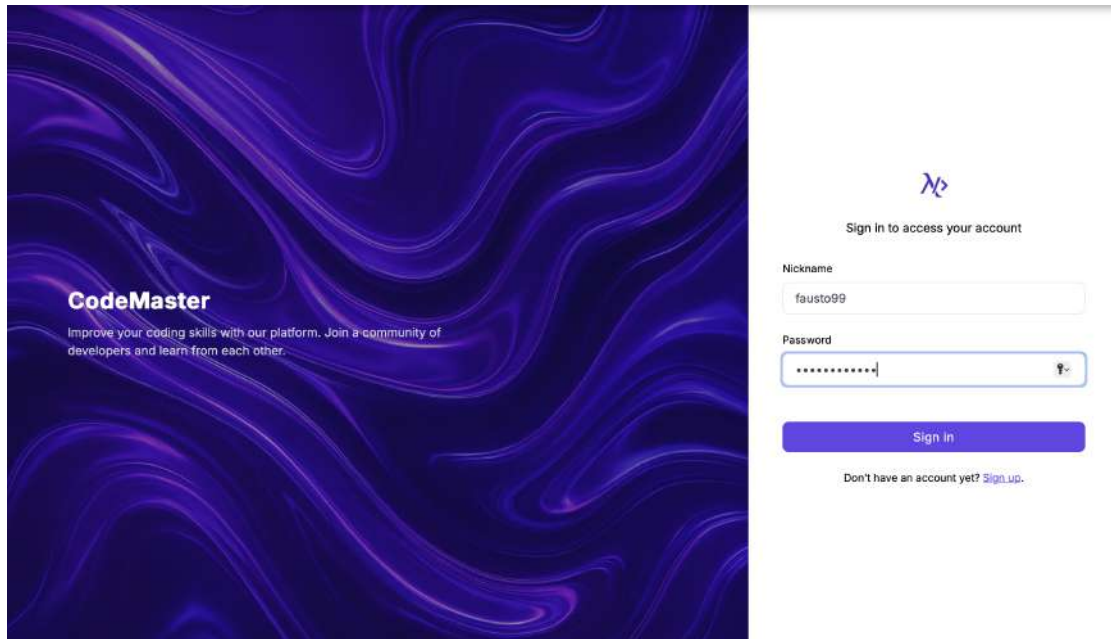
Figure 18: SignIn page
