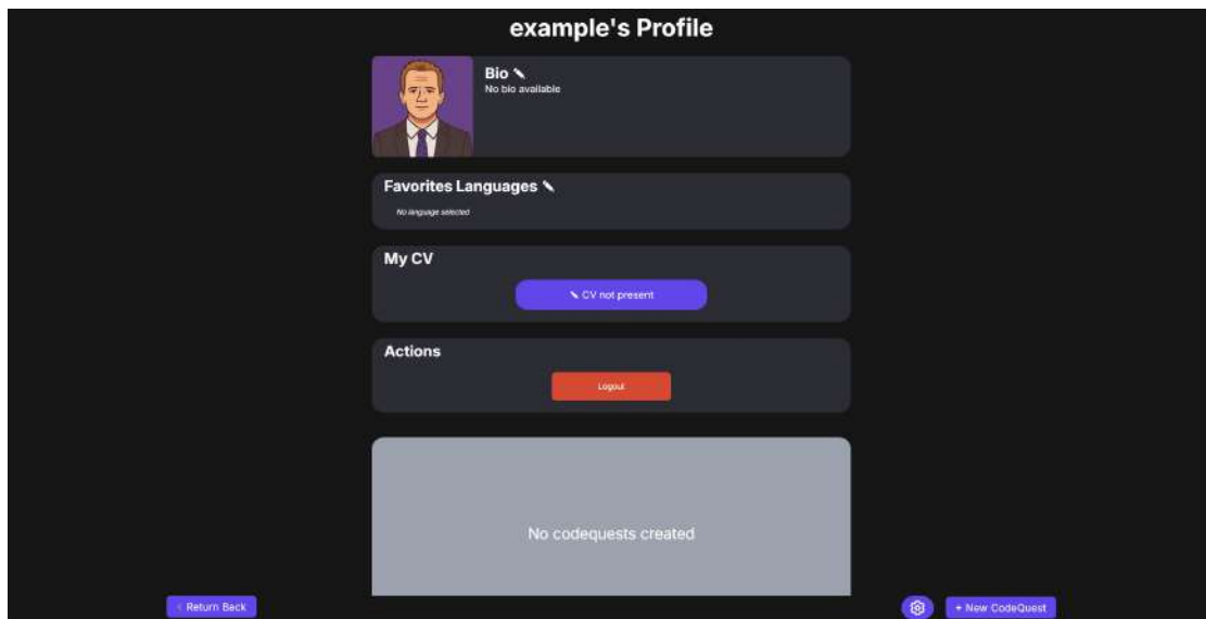
Figure 20: Profile
