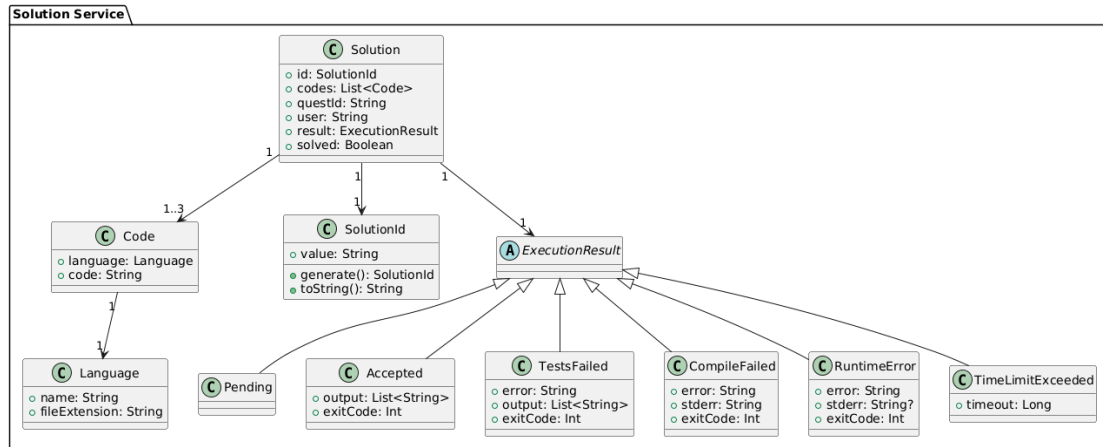
Figure 13: Solution class diagram
