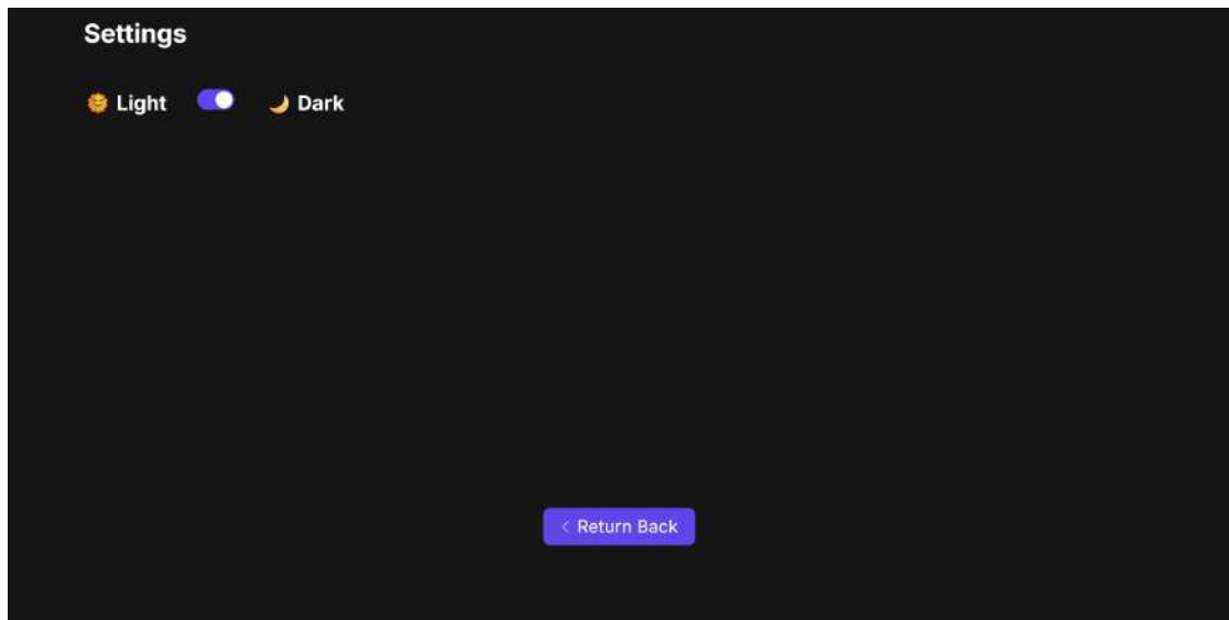
Figure 21: Settings page
