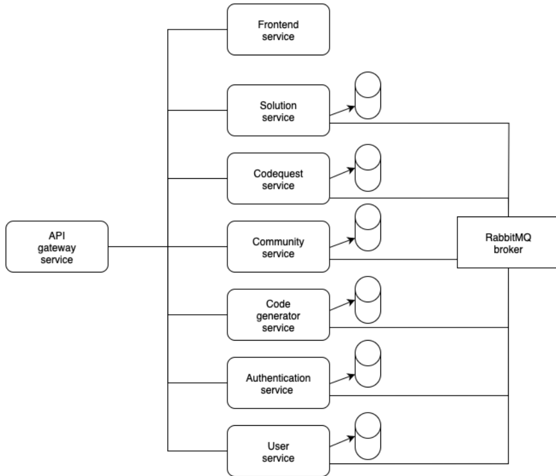
Figure 8: Codemaster infrastructure
