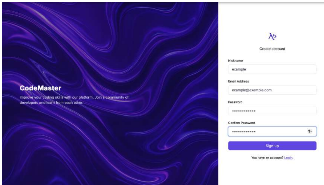
Figure 17: SignUp page
