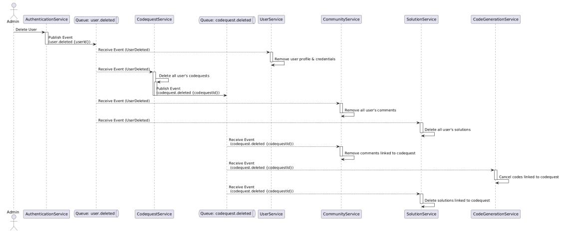
Figure 15: Delete User Sequence Diagram
