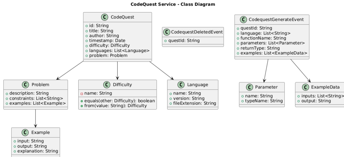
Figure 11: Codequest class diagram
