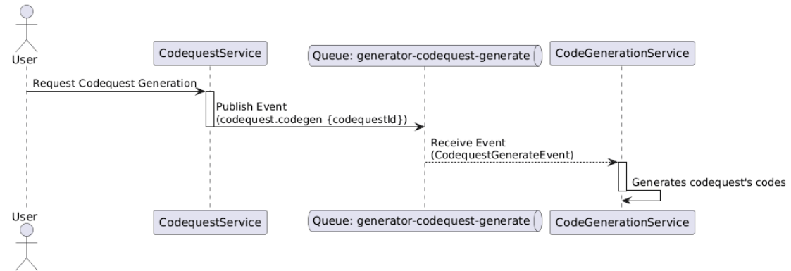
Figure 16: Code Generation Sequence Diagram
