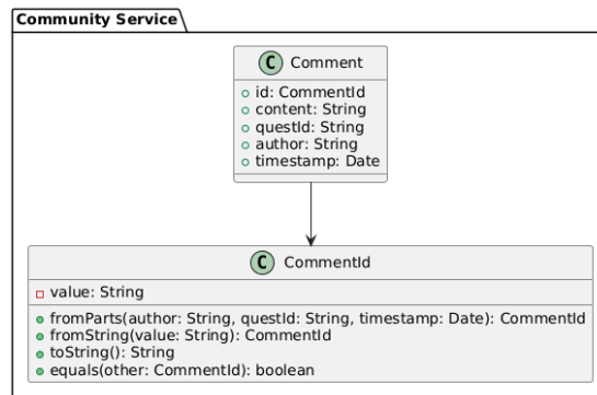
Figure 12: Community class diagram
