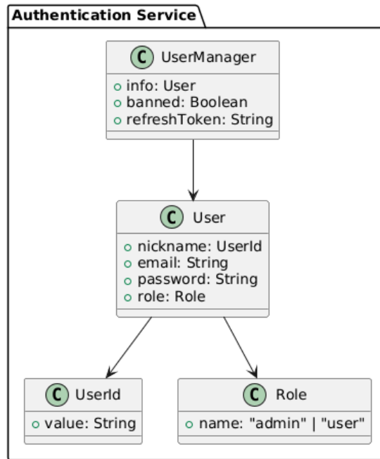
Figure 10: Authentication class diagram
