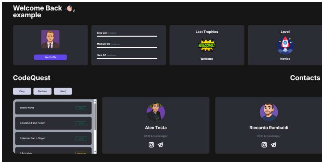
Figure 19: Dashboard page
