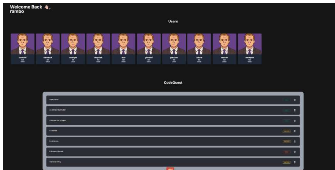
Figure 29: Admin section
