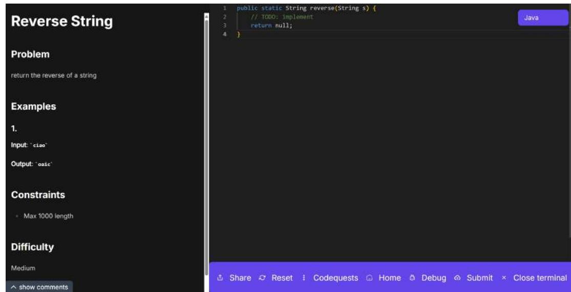
Figure 24: Codequest page
