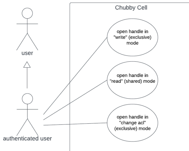
Figure 2: Use case diagram, operations that an authenticated user can do Upon authenticating, clients may open handles on nodes to execute specific operations afterwards
