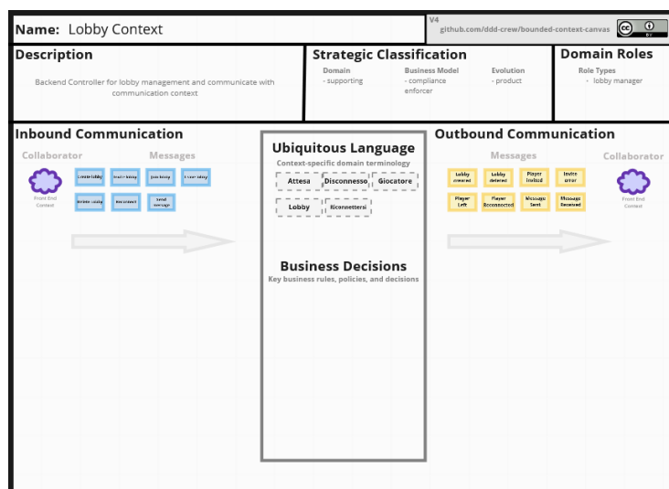
Figure 20: Bounded Context Canvas relativo alla lobby
