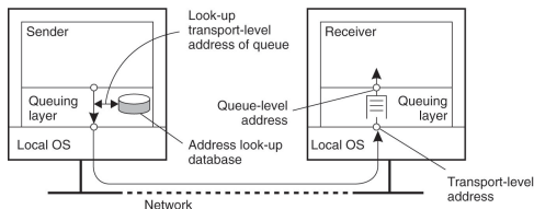
General architecture of a message-queuing system [Tanenbaum and van Steen, 2007]
