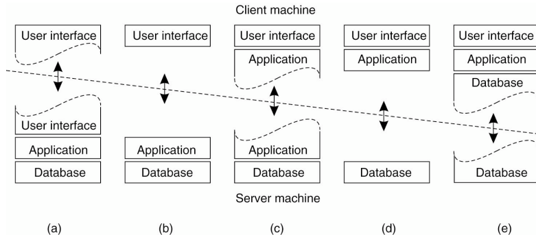
Alternative client-server organisations [TvS07]
