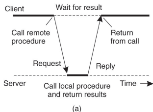
Traditional RPC
