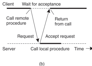
Asynchronous RPC
