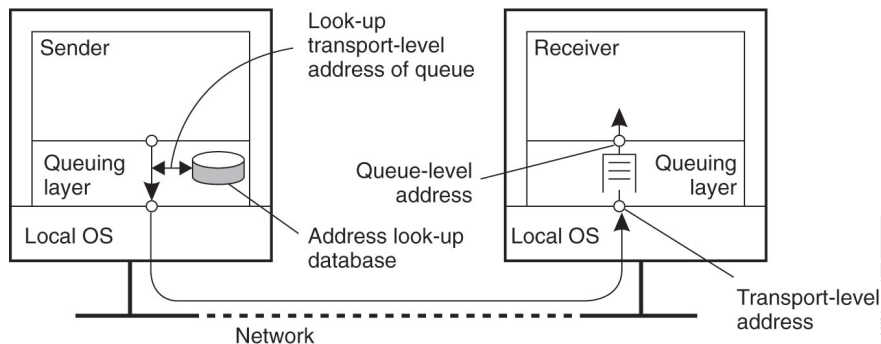
General architecture of a message-queuing system [TvS07]
